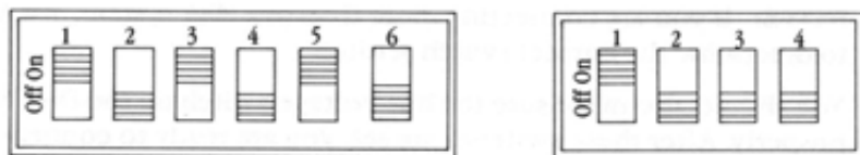
Figure 3-12. Switch Settings for Epson Printers
