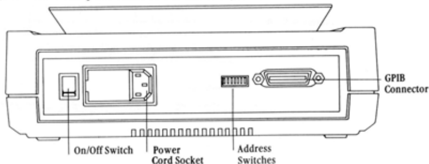
Figure 3-18. Rear View of the Hewlett-Packard ThinkJet Printer
