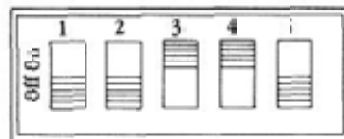
Figure 3-10 Switch Settings for Portable Diskette Drive
