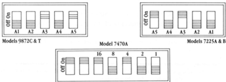
Figure 3-17. Switch Settings for Hewlett-Packard Plotters
