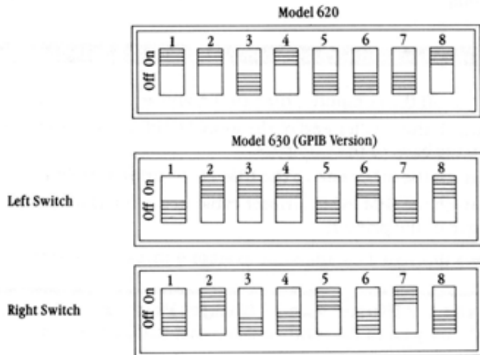
Figure 3-15. Switch Settings for Diablo Printers
